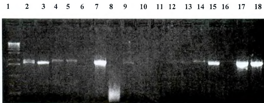
Figure 3. PCR amplification of phytoplasma DNA from diseased parthenium and reference samples in faba bean phyllody phy to plasma (FBP) and sunnhemp (SUNHP) phyllody phy to plasma using primers P1 and P7.
